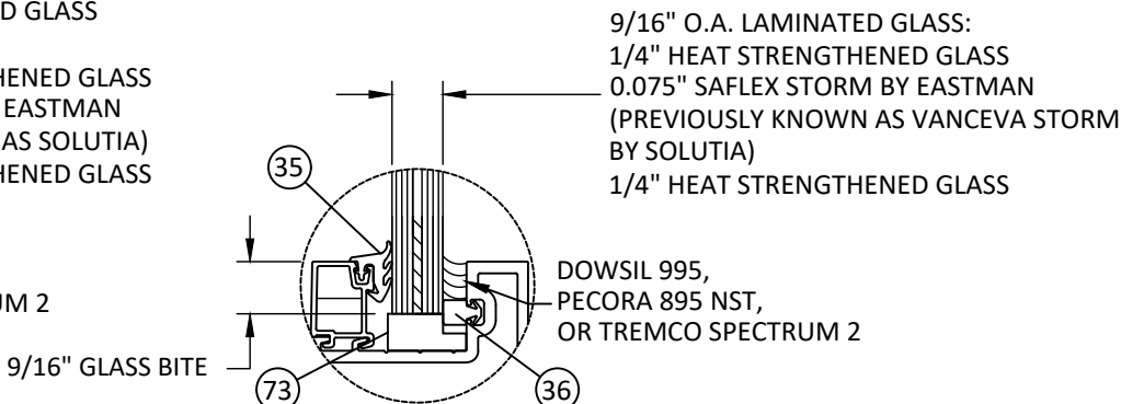
GLAZING DETAIL A1
