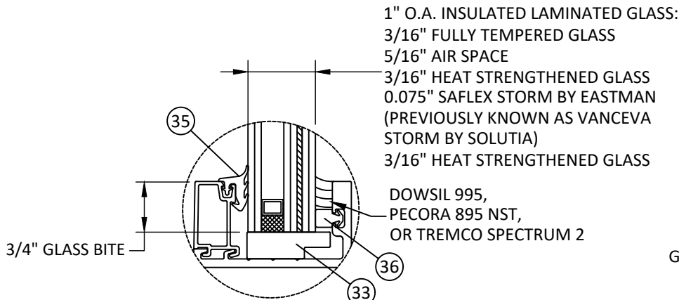
GLAZING DETAIL A
