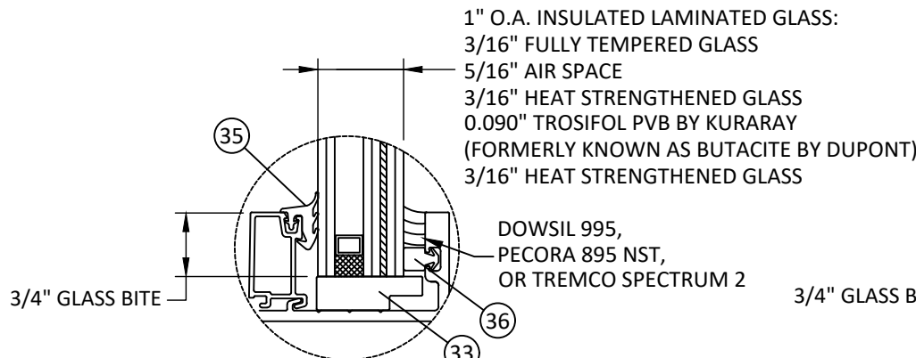
GLAZING DETAIL D
