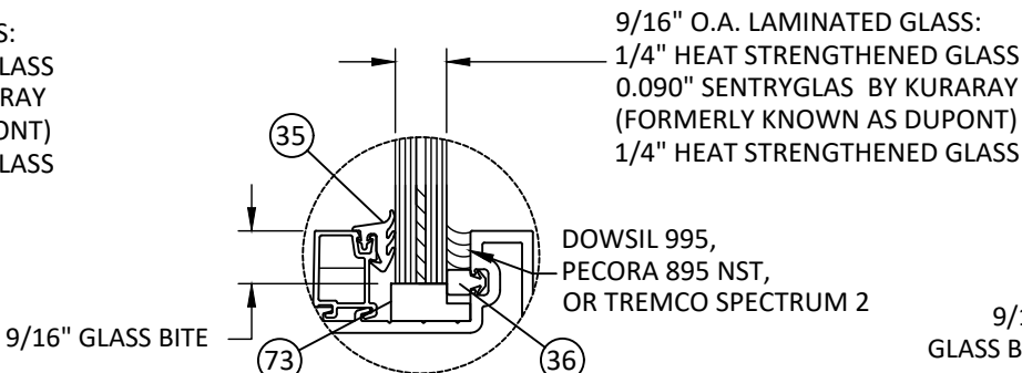
GLAZING DETAIL C1
