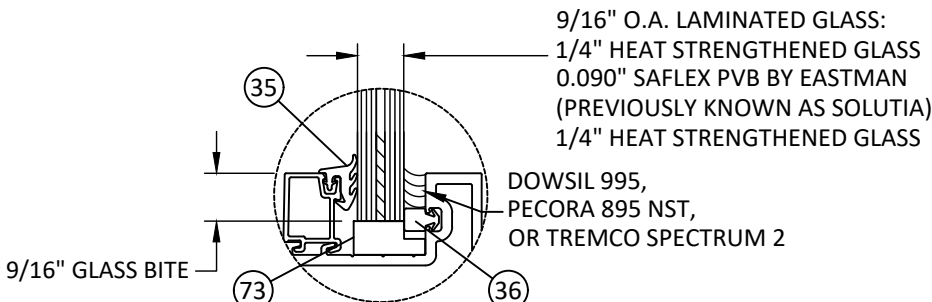
GLAZING DETAIL E1
