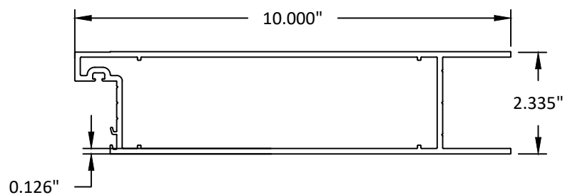
71 THRESHOLD RAMP 6063-T5
