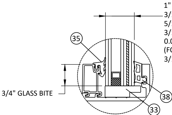
GLAZING DETAIL K DRY GLAZED
