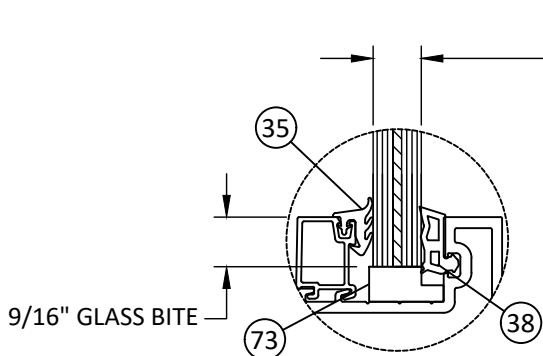
GLAZING DETAIL K1 DRY GLAZED
