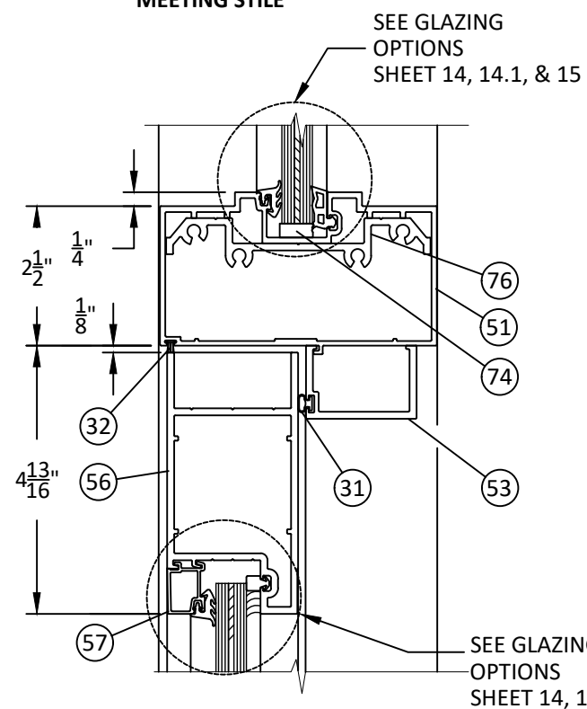
Q9 HORIZONTAL SECTION MEETING STILE
