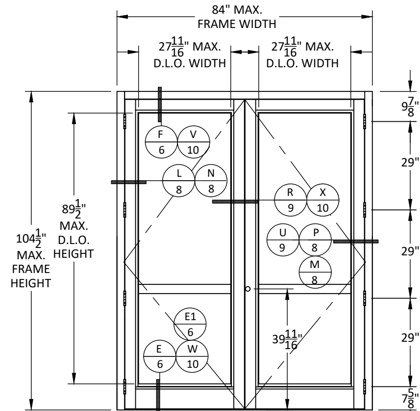
ELEVATION L RIM PANIC WITH REMOVABLE MULLION
