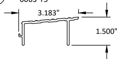
72 THRESHOLD RAMP 6063-T5
