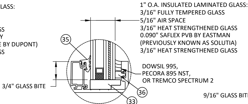
GLAZING DETAIL E
