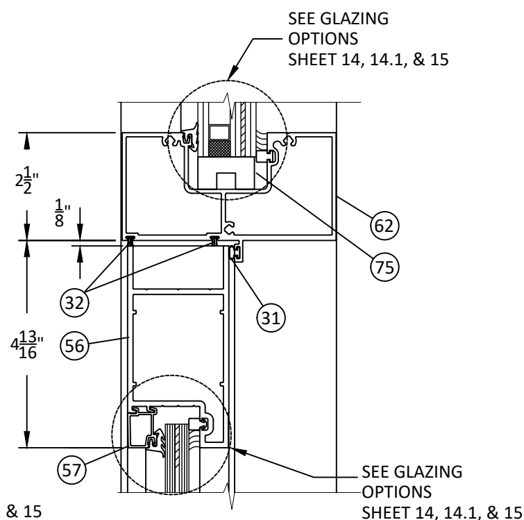
U9 HORIZONTAL SECTION VERTICAL MULLION STOREFRONT SYSTEM
