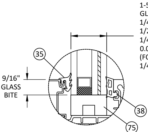
GLAZING DETAIL N DRY GLAZED TRANSOM
