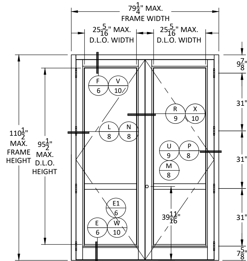
ELEVATION K RIM PANIC WITH REMOVABLE MULLION
