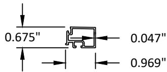
58 INT. GLASS STOP-MONO. 6063-T5
