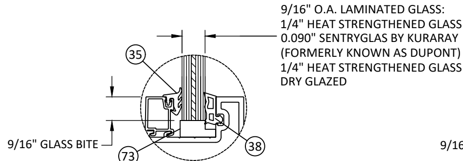
GLAZING DETAIL B1 DRY GLAZED
