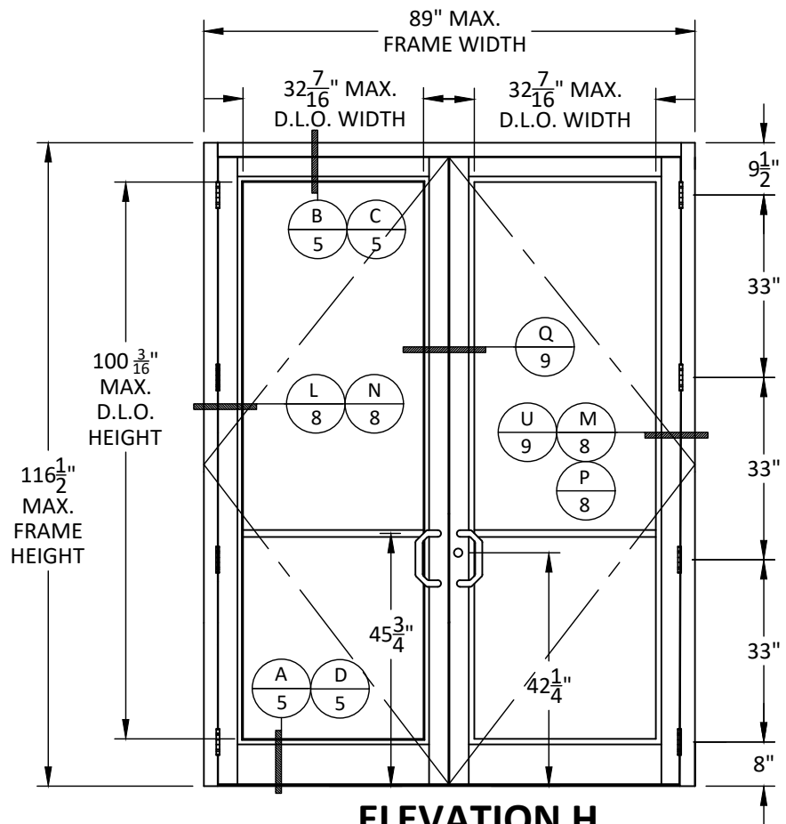
ELEVATION H STANDARD 5-POINT LOCK
