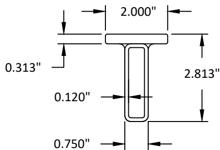
64 REMOVABLE MULL REINFORCEMENT STEEL
