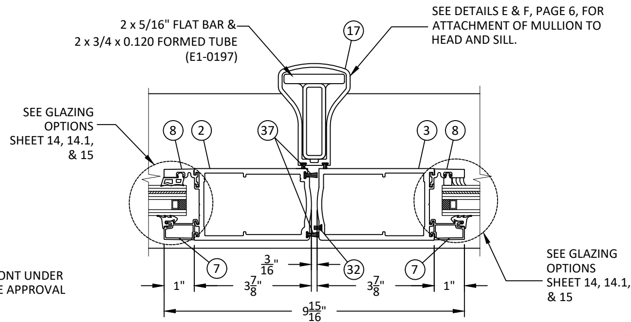
R9 HORIZONTAL SECTION MEETING STILE W/REMOVABLE MULLION
