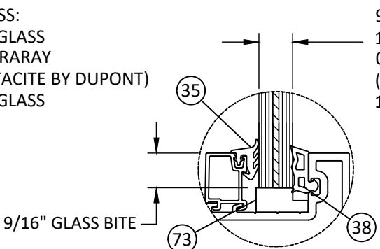
GLAZING DETAIL L1 DRY GLAZED
