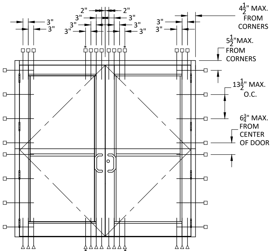
ANCHOR LAYOUT FOR ELEVATIONS A-E, H, I, K, & L
