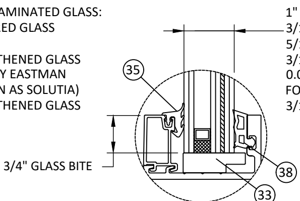
GLAZING DETAIL M DRY GLAZED
