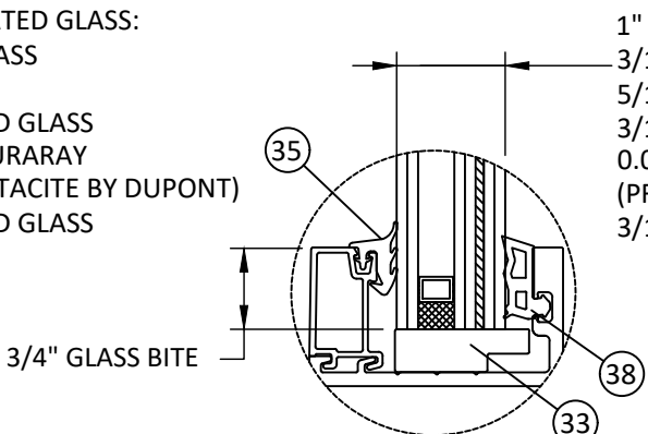
GLAZING DETAIL L DRY GLAZED
