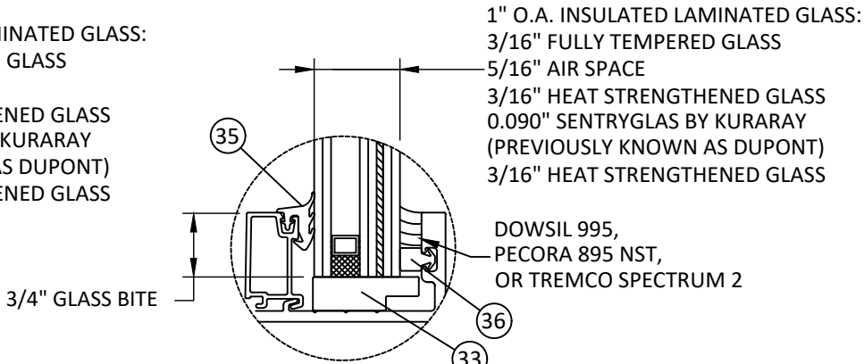
GLAZING DETAIL C
