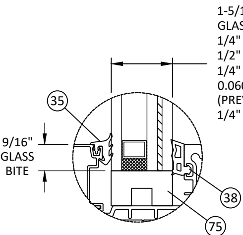
GLAZING DETAIL P DRY GLAZED TRANSOM
