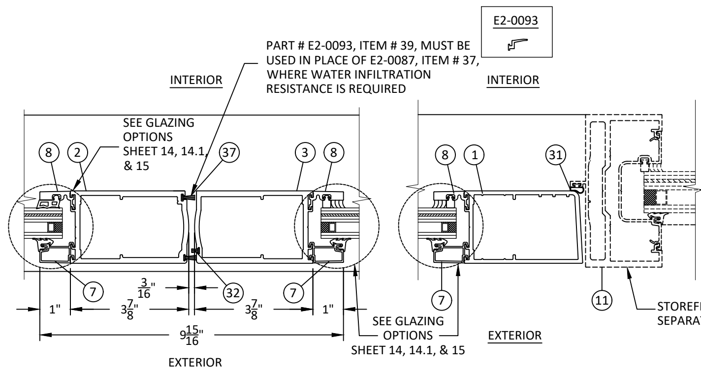
Q9 HORIZONTAL SECTION MEETING STILE
