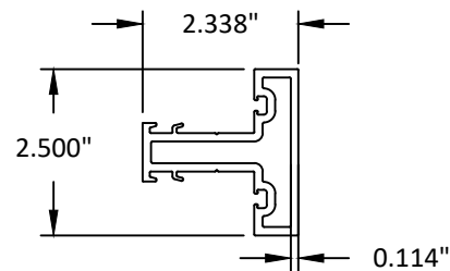
67 2 1/2" CROSS RAIL 6063-T5
