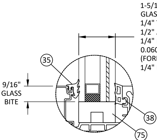
GLAZING DETAIL O DRY GLAZED TRANSOM
