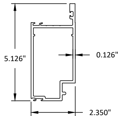
67 2 1/2" CROSS RAIL 6063-T5
