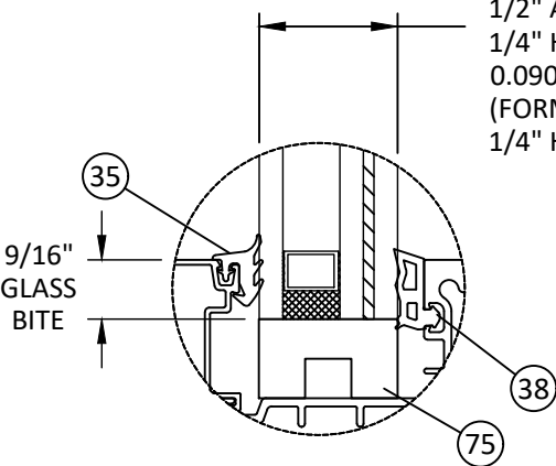
GLAZING DETAIL H DRY GLAZED TRANSOM
