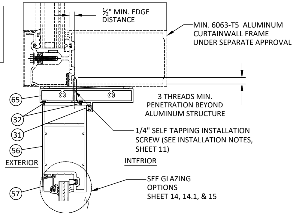
AB 12 VERTICAL SECTION HEAD - SUBFRAME TO CURTAINWALL OPTIONAL (STANDARD IN B/5)
