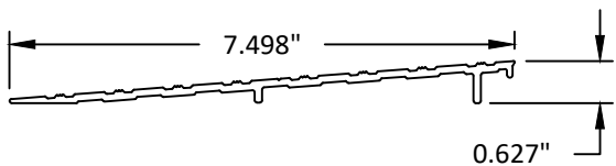
70 THRESHOLD RAMP 6063-T5
