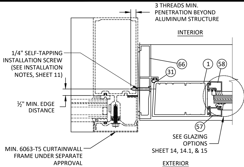
AA 12 HORIZONTAL SECTION JAMB - SUBFRAME TO CURTAINWALL
